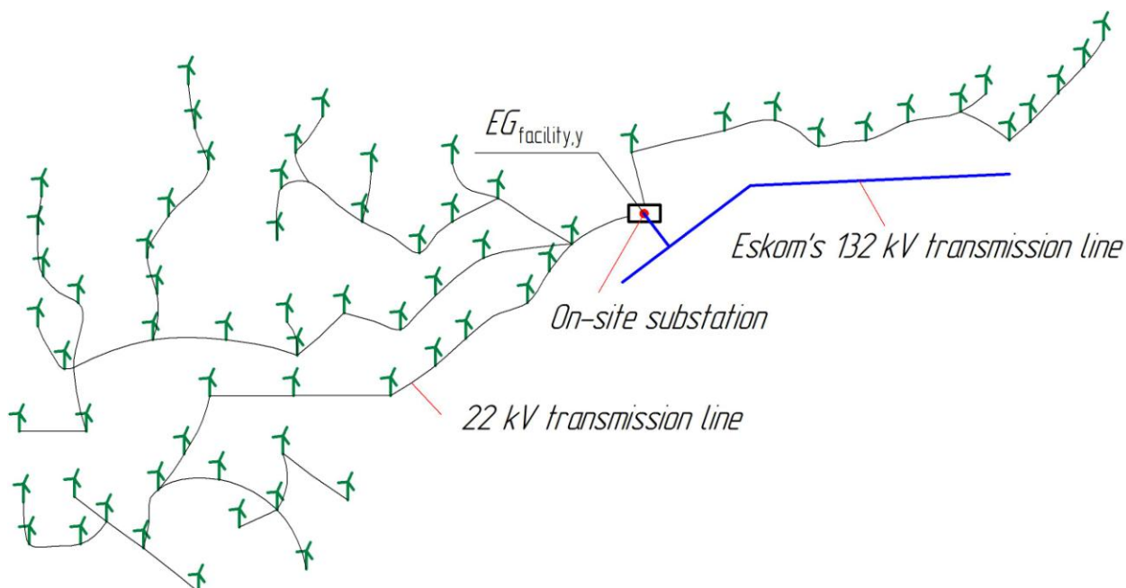
Fig. A.4-3: Basic diagram of the wind farm transmission network
